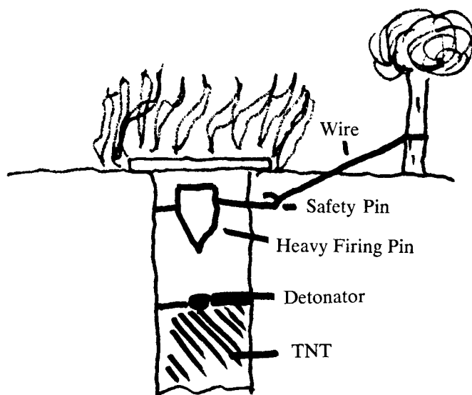
Figure 101. Walk trap.
