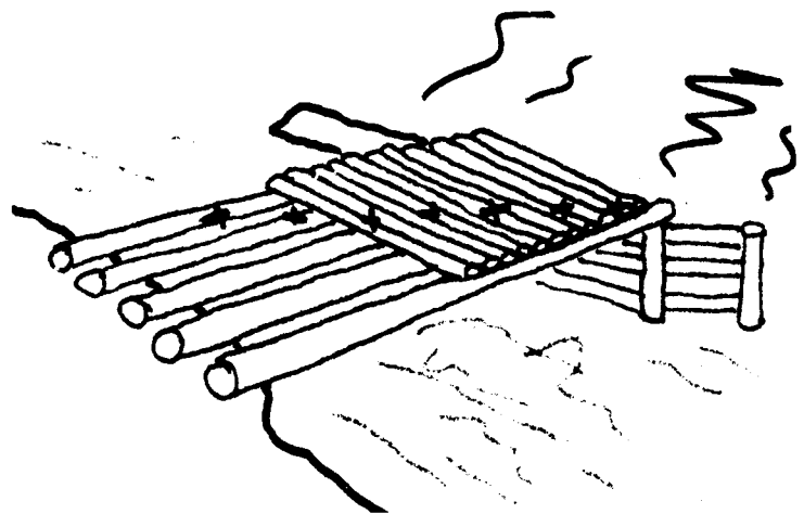
Figure 84. Slab bridge.
