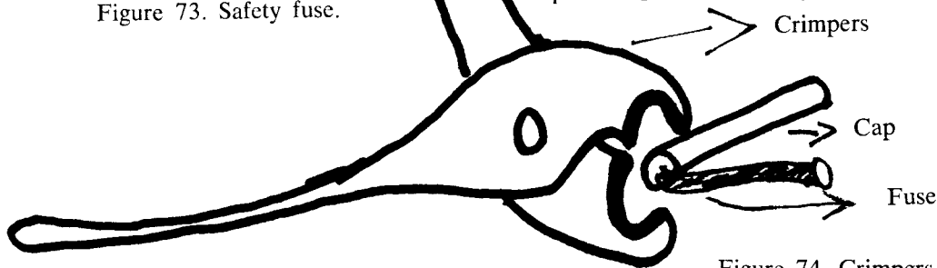
Figure 74. Crimpers.
