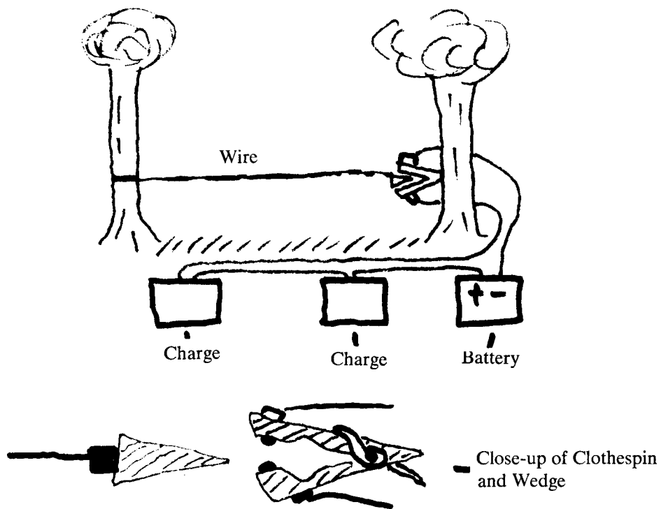
Figure 100. Road trap.
