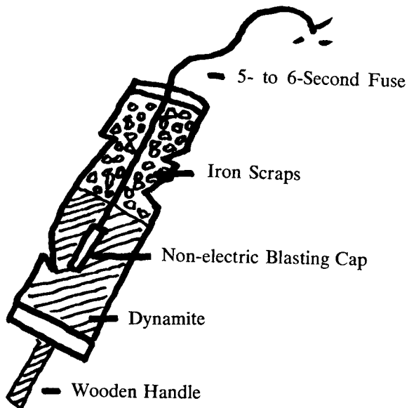
Figure 104. Homemade grenade.
