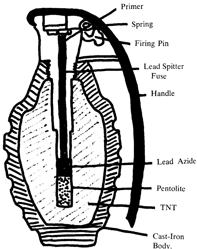
Figure 90. Military grenade.
