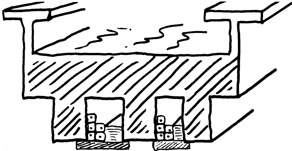
Figure 85. T-beam bridge.
