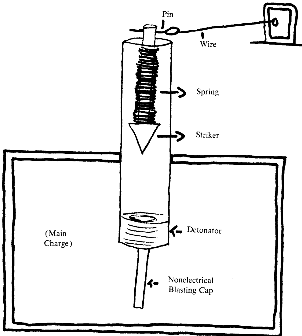
Figure 89. Tension-release detonator.
