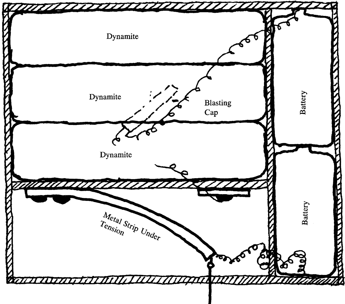
Figure 95. Tension-release detonator.
